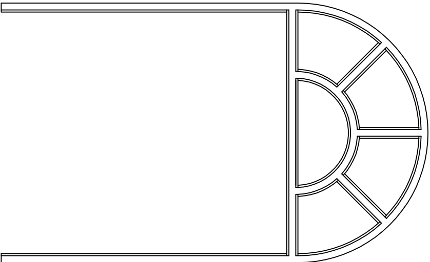
Round Top Frames w/ Interior Arched Mullion & Sun Burst
